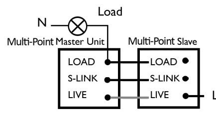
Fig 3. Alternative Wiring for Multi-Way Circuits
