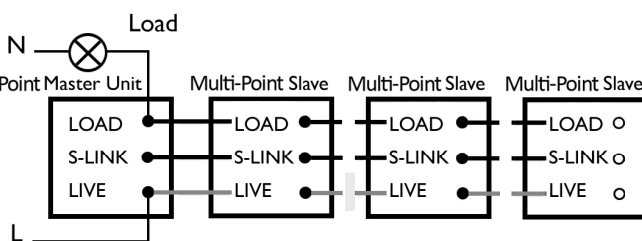
Fig 2. Wiring for Multi-Way Circuits
