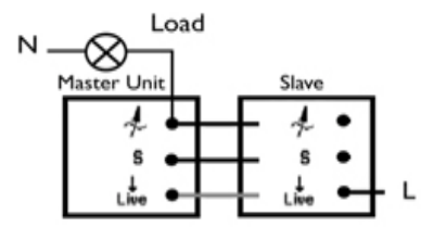
Fig 3. Alternative Wiring for Multi-Way Circuits
