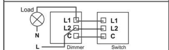
Figure 2. Using a 2-way dimmerswitch DIMMER MUST REPLACE ONLY ONE OF THE 2-WAY SWITCHES
