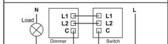
Figure 3. Using a 2-way dimmerswitch DIMMER MUST REPLACE ONLY ONE OF THE 2-WAY SWITCHES
