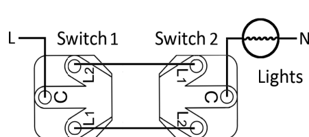
Two-way circuit (type 1)
