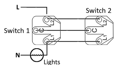
Two-way circuit (type 2)
