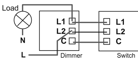
Figure 2. Using a 2-way dimmerswitch DIMMER MUST REPLACE ONLY ONE OF THE 2-WAY SWITCHES
