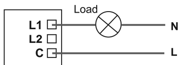
Figure 1. Using a 1 or 2-way dimmer switch
