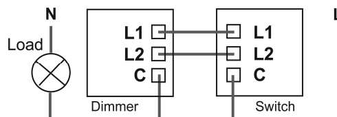
Figure 3. Using a 2-way dimmerswitch DIMMER MUST REPLACE ONLY ONE OF THE 2-WAY SWITCHES
