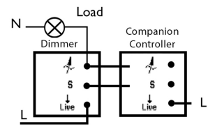
Fig 3. Alternative Wiring for 2 or 3-Way circuits
