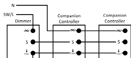
Fig 2. Wiring for 2 or 3-Way Circuits
