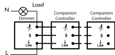
Fig 2. Wiring for 2 or 3-Way Circuits
